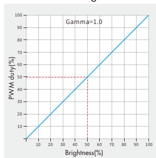
Dimming curve
