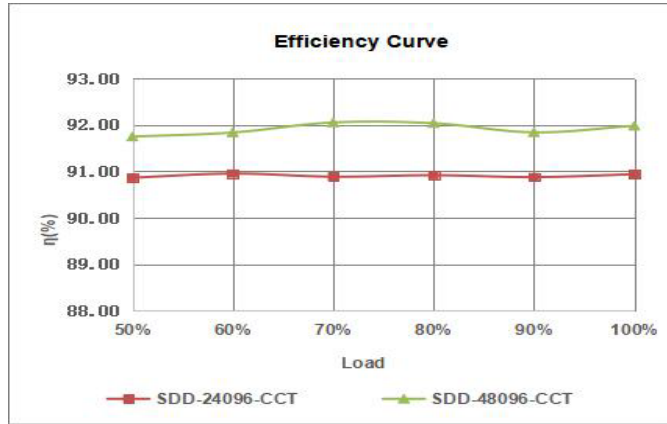
Efficiency Curve (efficiency vs output load)
