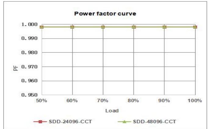
Power factor curve
