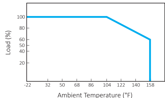
DERATING CURVE
