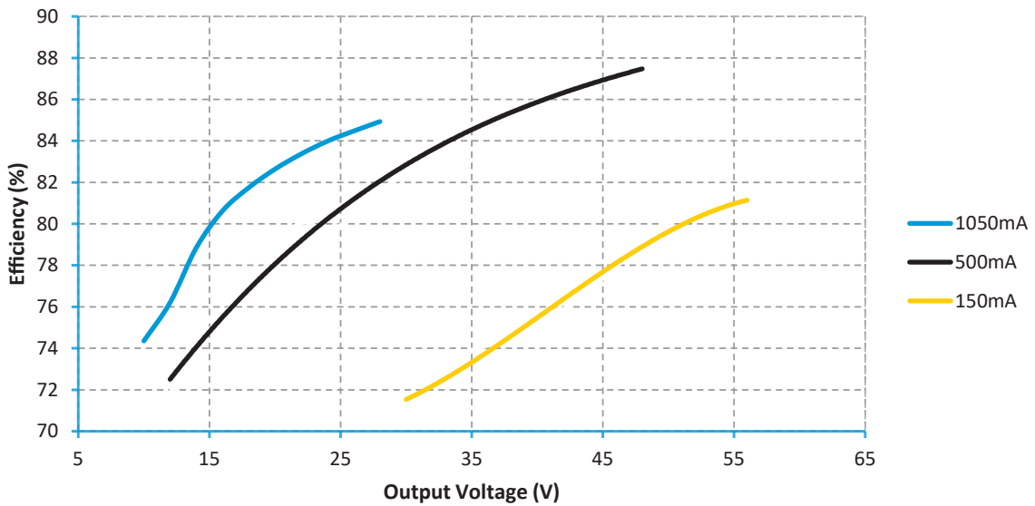
Efficiency @ 120V
