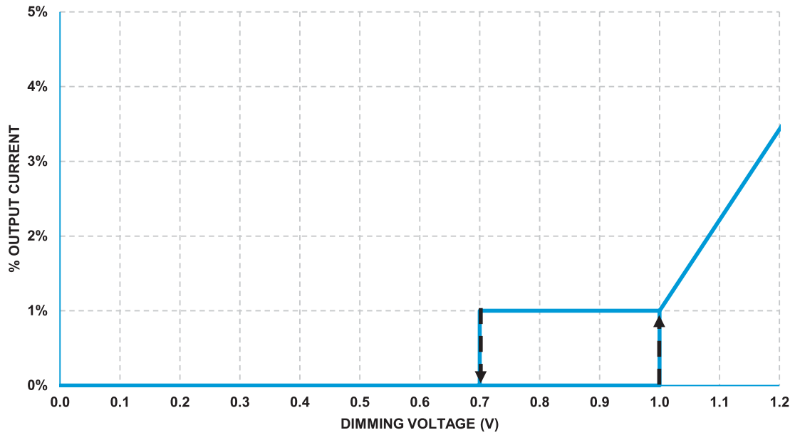
Dim-To-Off Hysteresis
